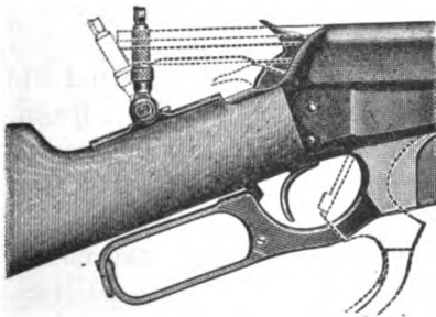
Regular base flexible sight on rifle with long firing bolt
