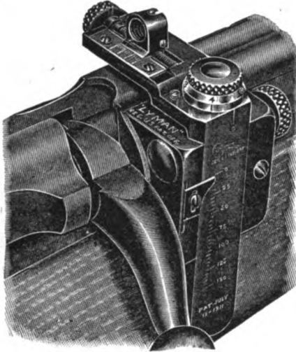
Fig. 56 Lyman No. 48 receiver sight for Springfield rifle
