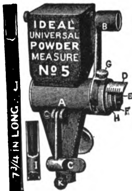
Fig. 82 Ideal universal powder measure No. 5
