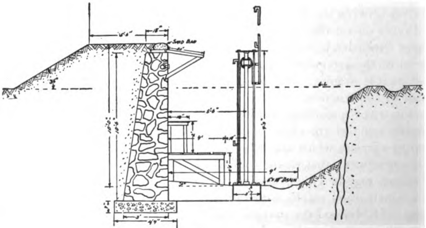
Profile of rifle range butt, showing construction. Dimensions correct for commercial steel target carrier
