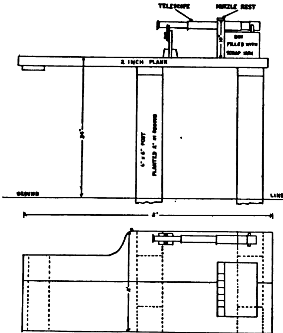
Fig. 152 Details of muzzle and elbow rest table. Side and top views
