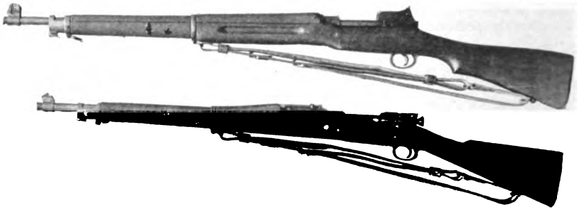
Fig. 25 The United States rifles. View of left side Upper — Model 1917 Lower — Model 1903
